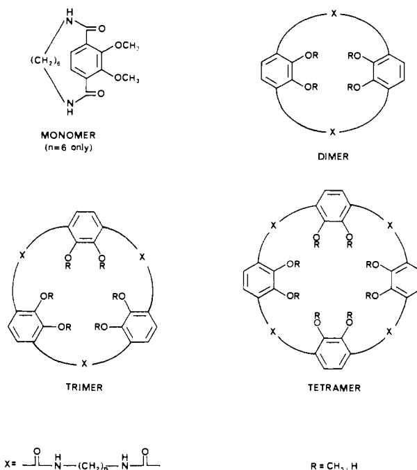
Figure 1. High-dilution synthesis of polycatecholate macrocycles.
